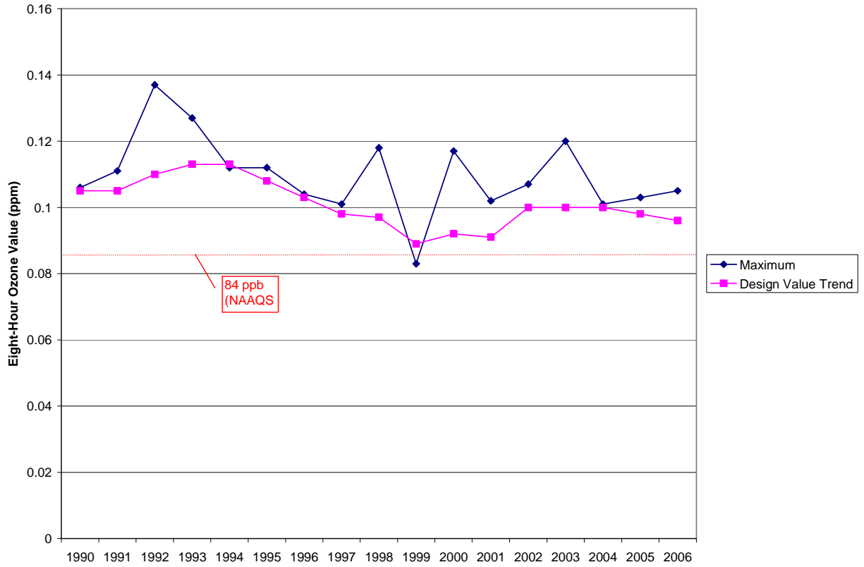
Figure 1 - Federal 8-Hour Ozone Design Value Trend
