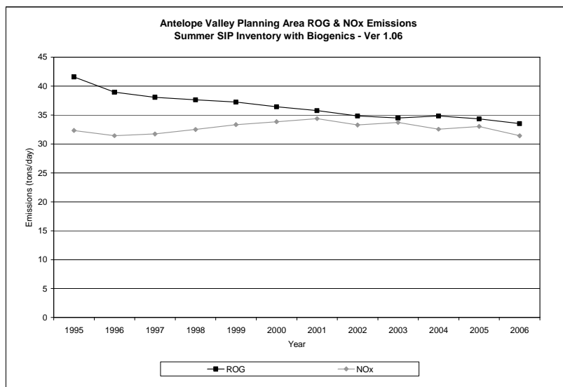
Figure 8: Antelope Valley Estimated ROG and NOx Emissions 1995 to 2006
